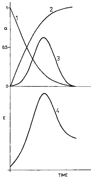
Fig. 3 Isothermal kinetic curves of thermal decomposition reaction of a solid sample based on the 'three-component model'. Curves 1, 2 and 3 describe changes of the amount of the respective components 1, 2 and 3 in the sample; curve 4 describe changes of the emanation power E of the sample labelled uniformly by the radon parent nuclide. Following parameters were used in the modelling: A=0.25 , K=2.2 , T_m=2.2 , E_1=0.04 , E_2=1.0 , E_3=0.4
